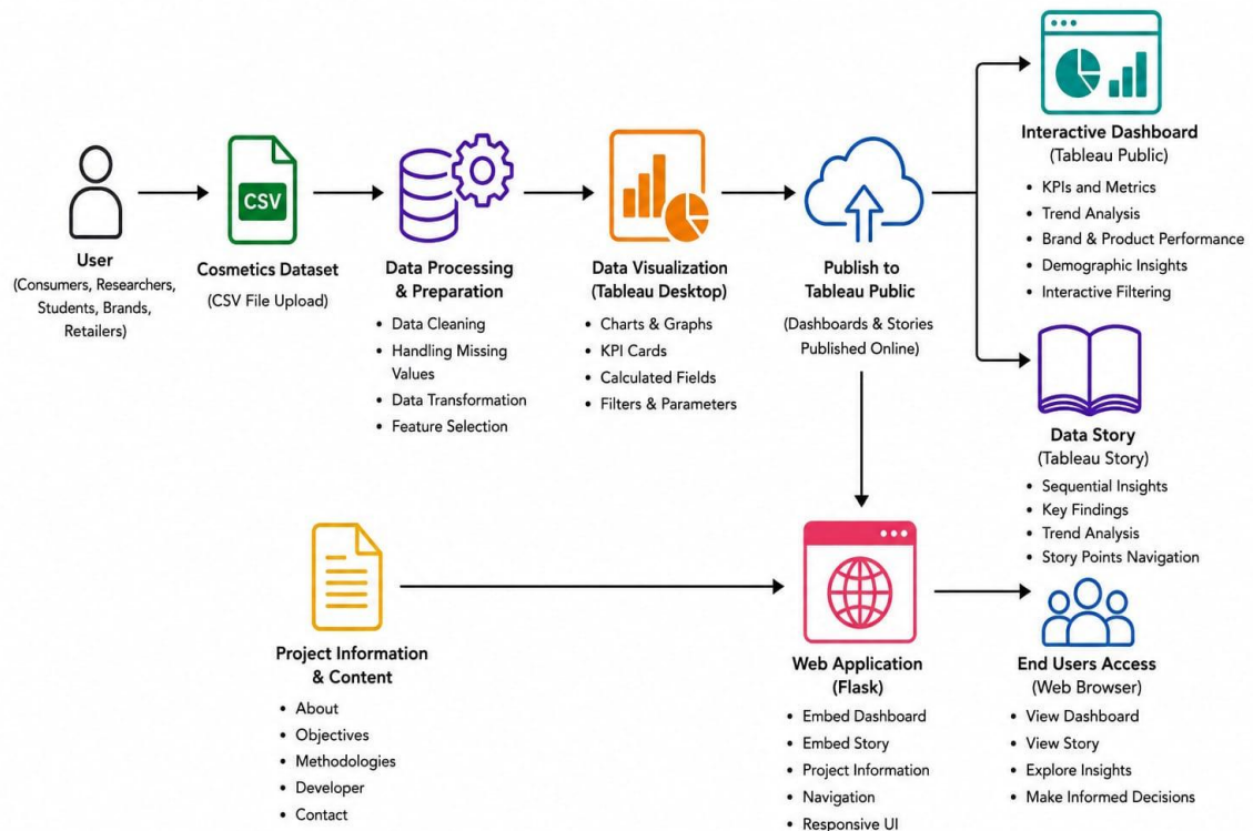
Figure 1: Architecture and data flow of the Cosmetic Insights application
